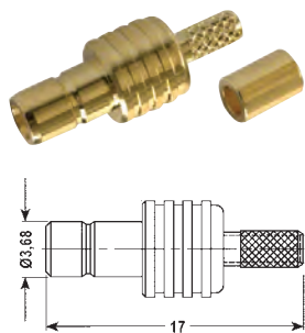
Art. SB/1245 per cavo RG174 50ohm
