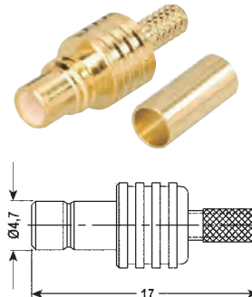
Art. SBC/110 per cavo RG174 50ohm
