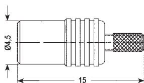
Art. MCX/150 per cavo RG174 50ohm
