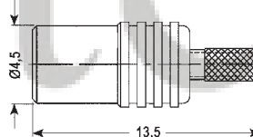
Art. MMCX/220 per cavo RG174 50ohm
