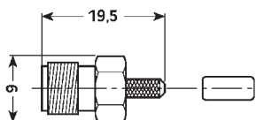
Art. S/1258 per cavo RG58 50ohm
