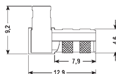
Art. MCX/130 per cavo RG174 50ohm
