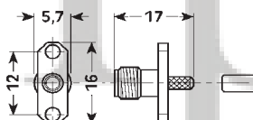
Art. S/1253 per cavo RG58 50ohm
