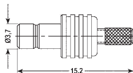
Art. MCX/100 per cavo RG174 50ohm
