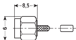
Art. S/1250 per cavo RG58 50ohm
