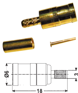
Art. SB/1240 per cavo RG174 50ohm
